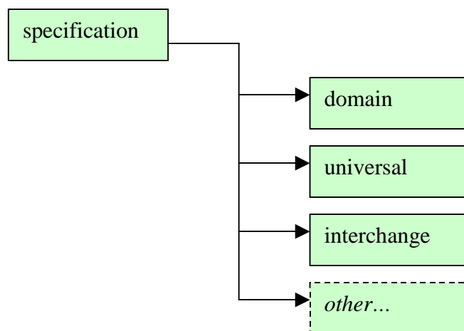
Figure 6: Specification hierarchy
