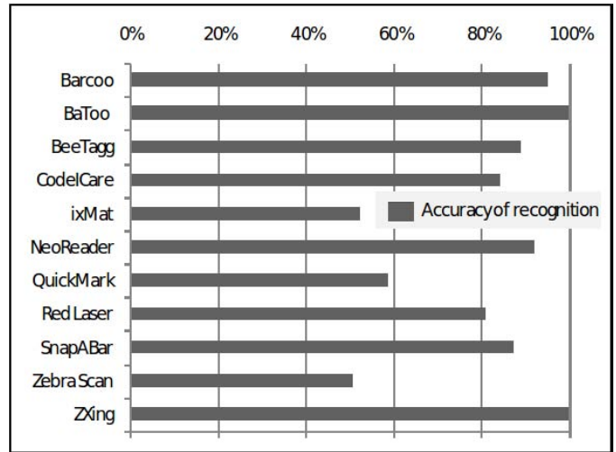
Fig. 5. Reliability of recognition by scanner
