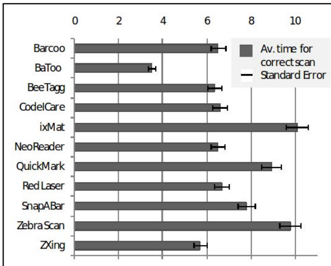
Fig. 6. Average task completion time by scanner
